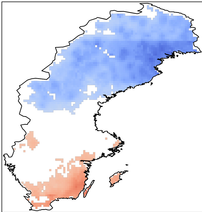
Drought index and corn yield
